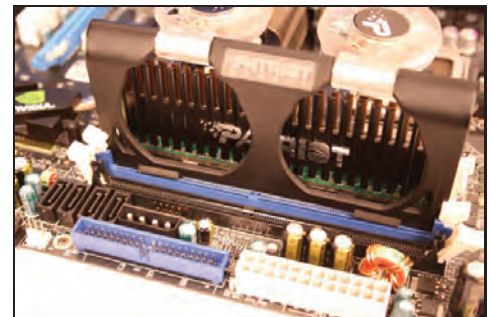
Photos show Vortex's unique dimm slot installation/mounting design.
